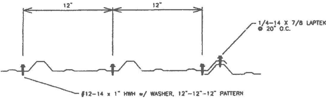
FASTENER PATTERN FOR INTERIOR SUPPORTS
